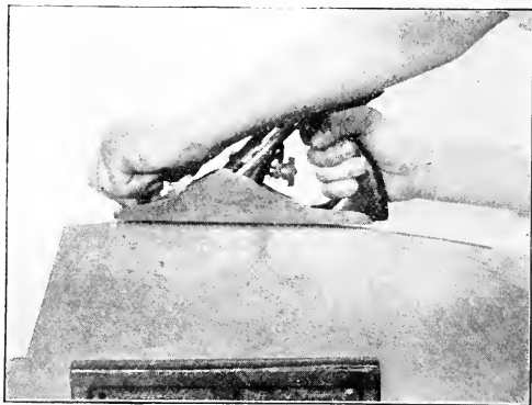
Fig. 159—Planing Curve
